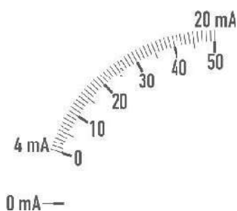
Scala a zero vivo (standard) Live zero scale (standard)
